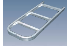
Folding nose extension 20" long F2 - For Cast Noses 220346 F2E - For Extruded Noses 220082 30" long F3 - For Cast Noses 220343 F3E - For Extruded Noses 220083
